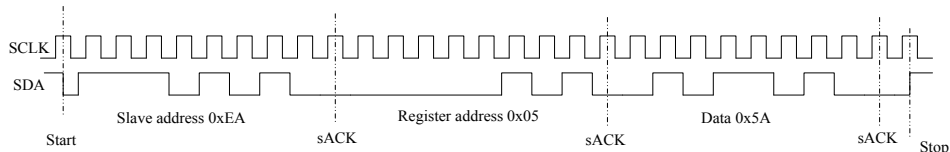
I2C WRITE
